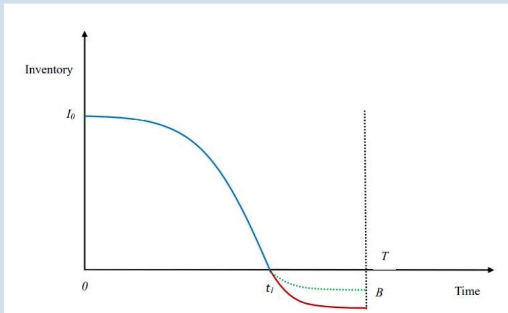
Figure 1. Inventory level.
